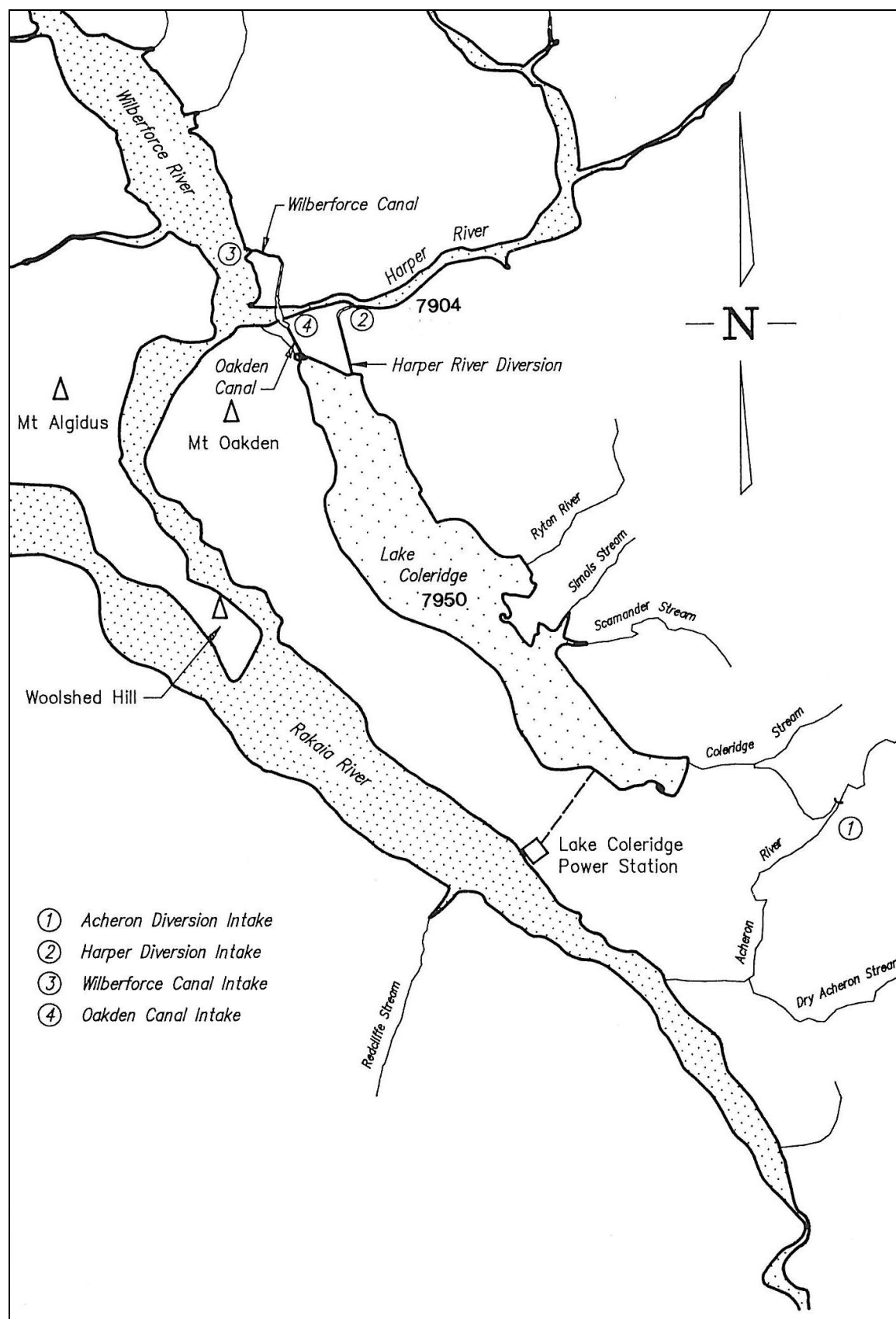
Figure 4.12 Layout of Coleridge Power Scheme
