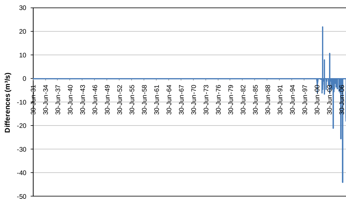
Figure 6.17 165101 (1) Hurunui SH1 Bridge data differences plot
