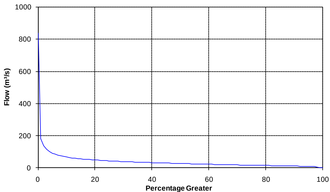
Figure depicting percentage exceedance graph
