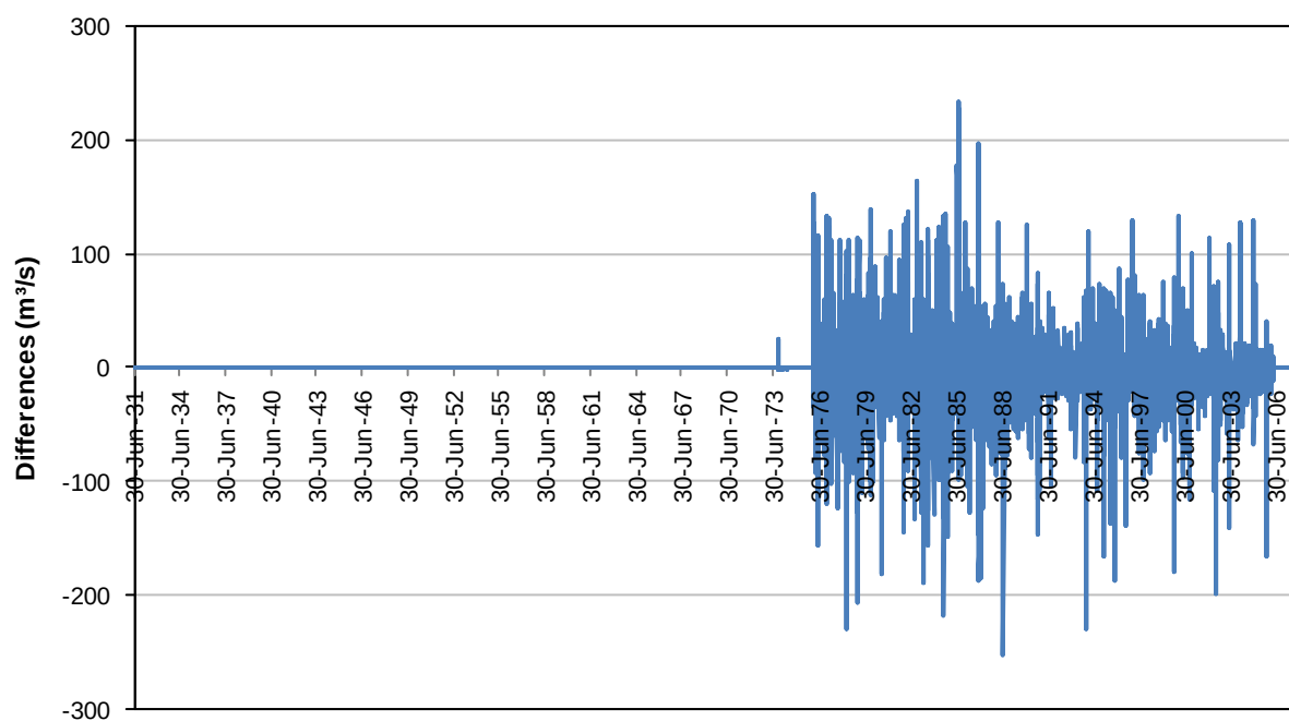
Figure 6.5 99552 (1) Manapouri data difference plot
