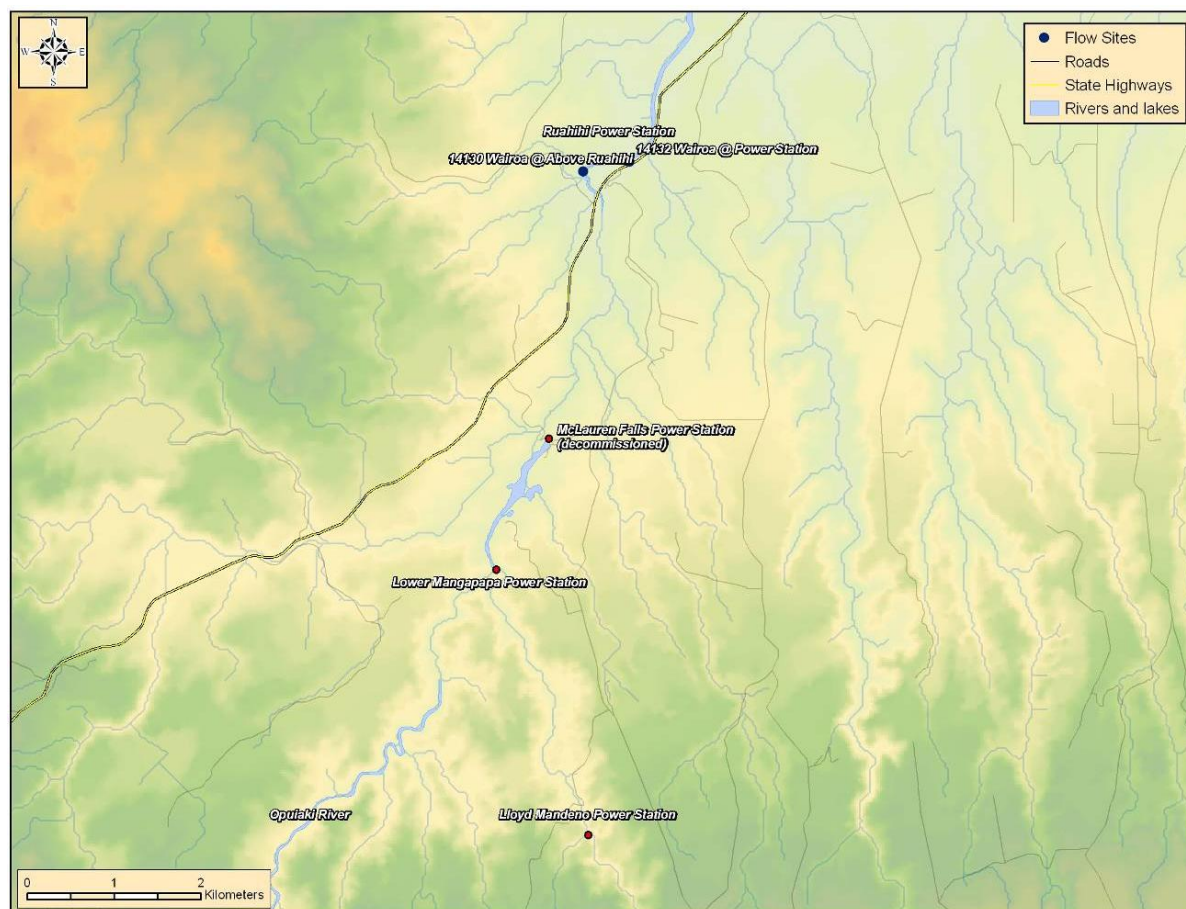
Figure 4.28 Kaimai Hydro Power Scheme location diagram
