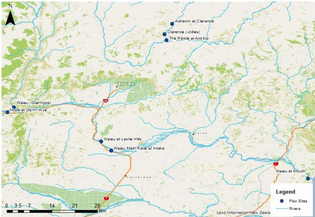
Figure 3-12: Wairau River location diagram.
