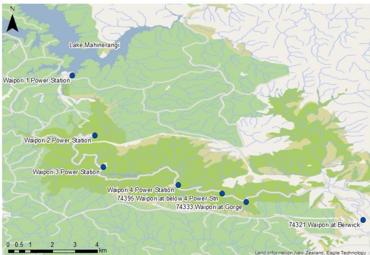
Figure 3-10: Waipori Power Scheme and gauging station location diagram.
