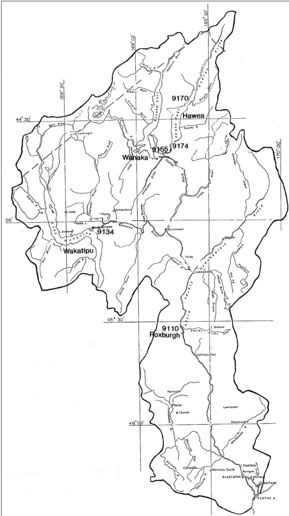
Figure 3-6: Clutha catchment.
