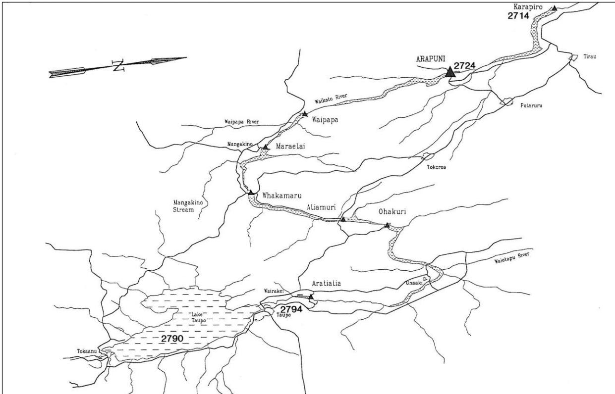
Figure 2-2: Waikato Power Development.
