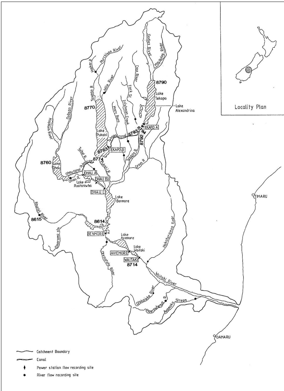
Figure 3-2: Waitaki hydro scheme.
